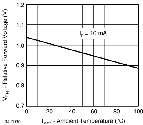
Fig. 2 - Relative Forward Voltage vs. Ambient Temperature
